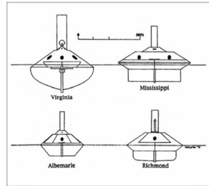
A comparison of Confederate ironclad hull types (drawing K. Blomquist)
